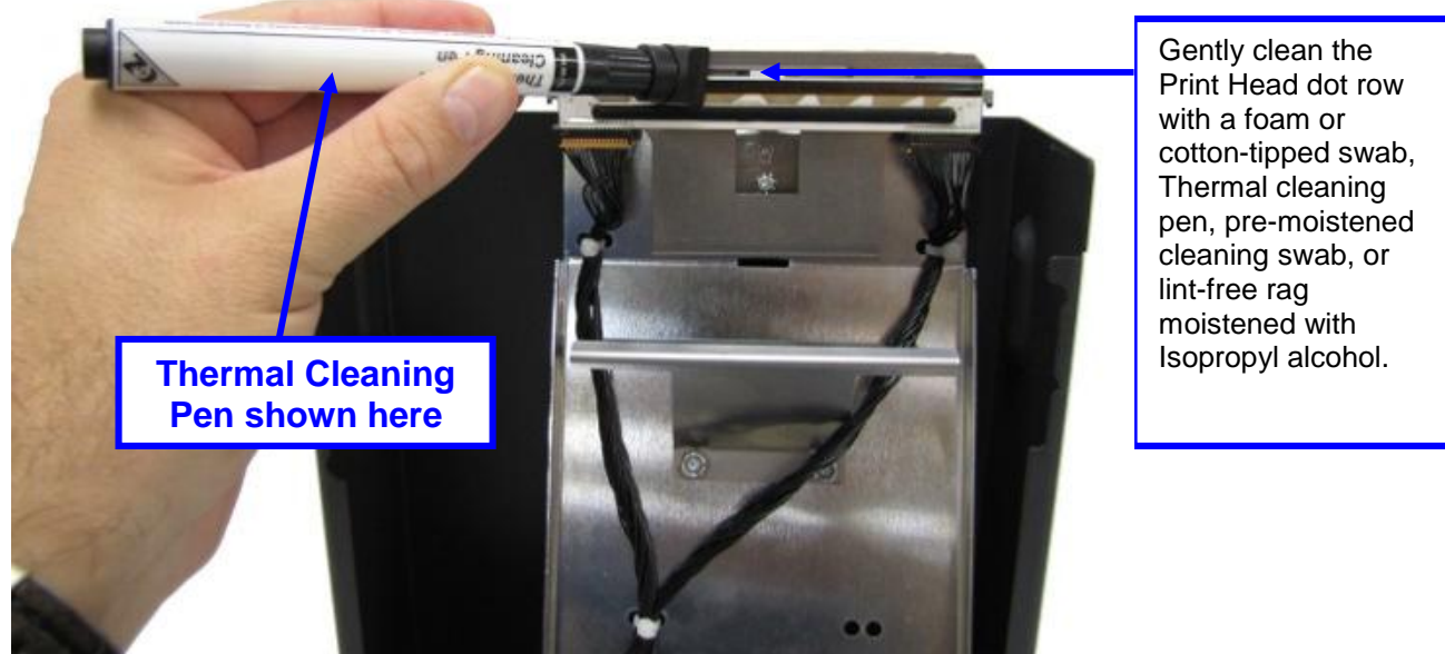
Figure 10-3 Cleaning the Print Head
