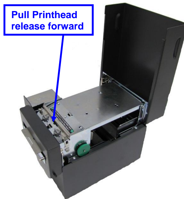
Figure 3-5 Printhead release
