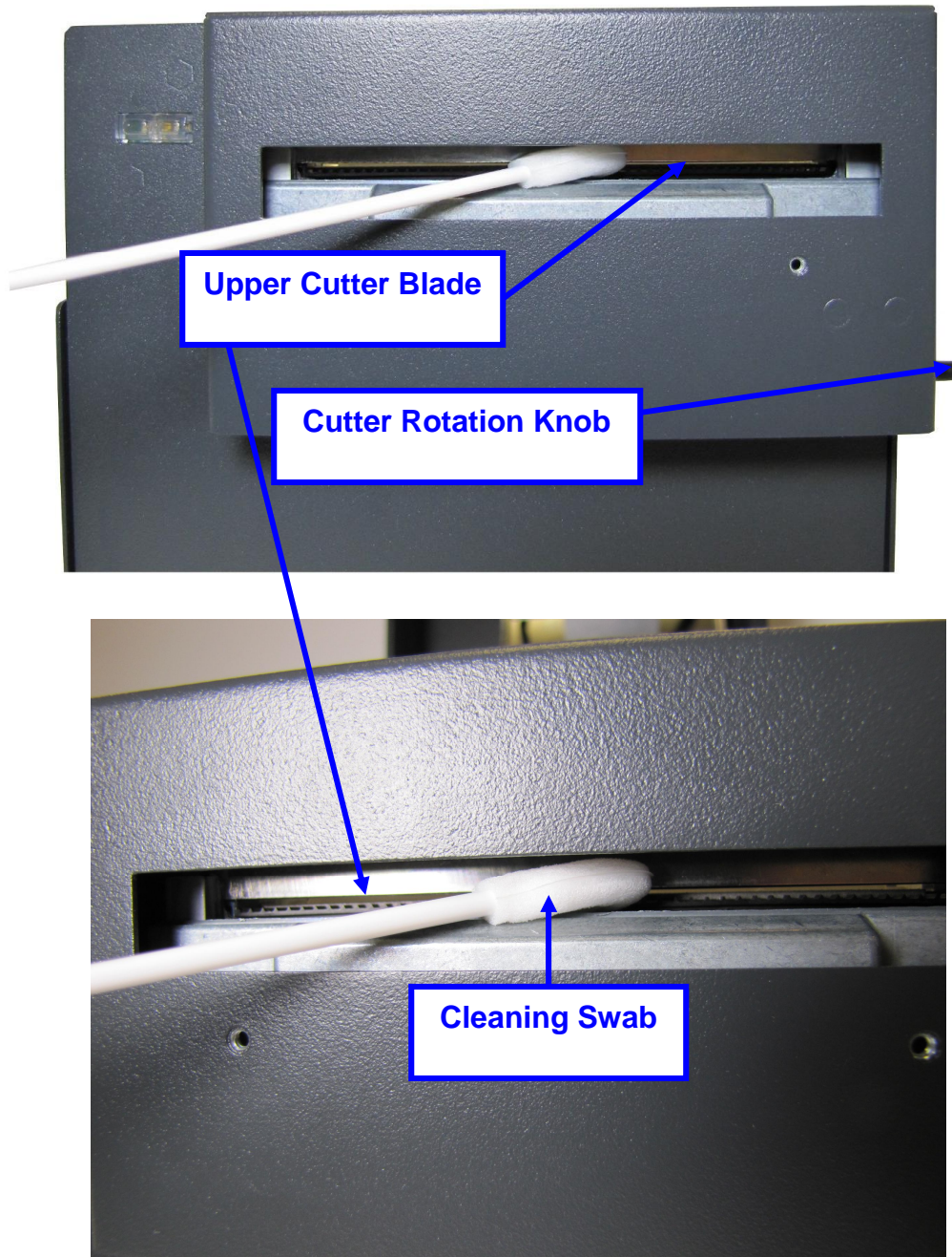
Figure 10-5 Cleaning the Upper Cutter Blade
