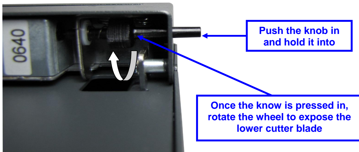
Figure 10-6 Cutter Rotation Knob
