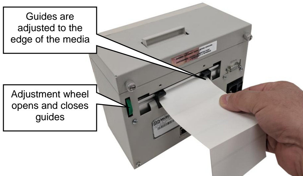
Figure 3-5 Loading Media – Adjustable Guide
