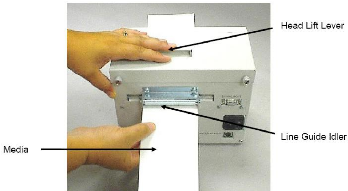
Figure 3-4 Loading Media – Fixed Guide
