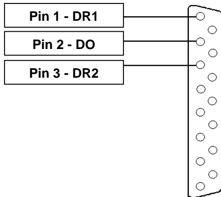
Figure 3-3 Cash Drawer Pin-out
