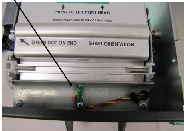
Figure 3-9 TOF (Top-Of-Form) Sensor
