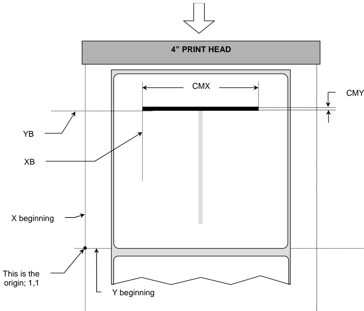
Figure 4-6 Label Format Line Draw
