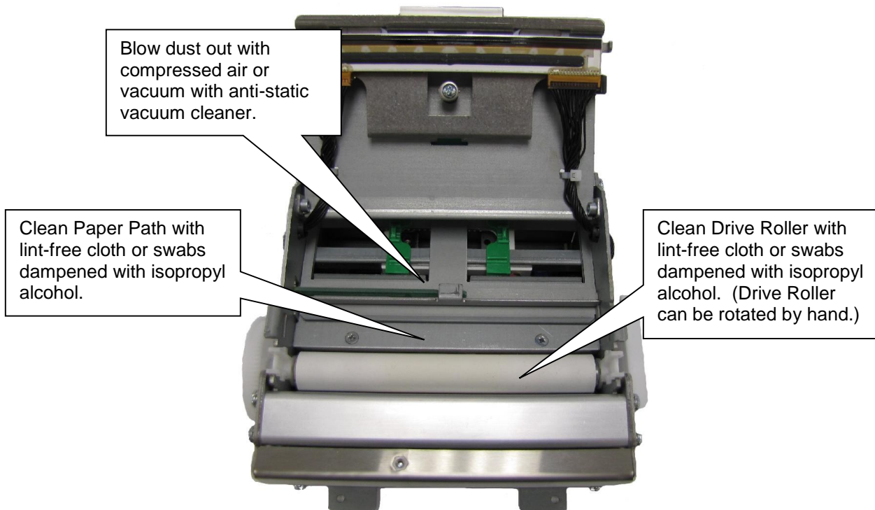
Figure 10-4 Internal Cleaning
