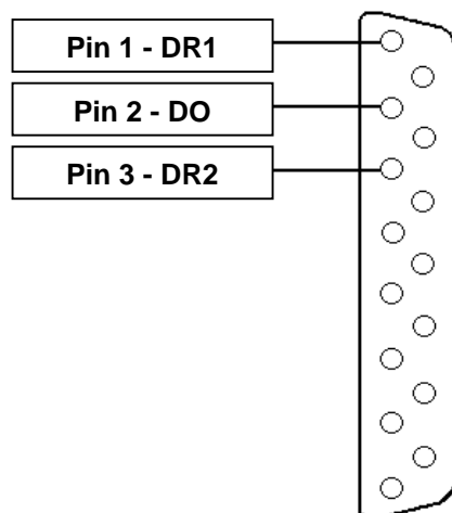
Figure 3-3 Cash Drawer Pin-out
