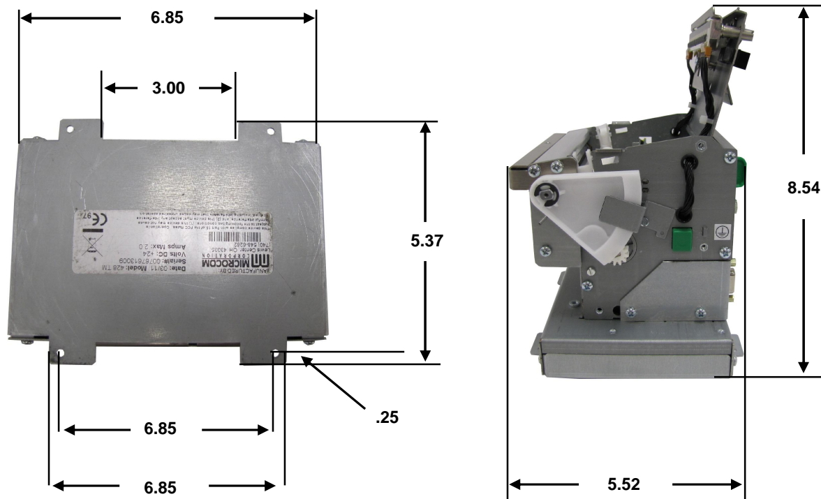
Figure 3-9 Printer Dimensions
