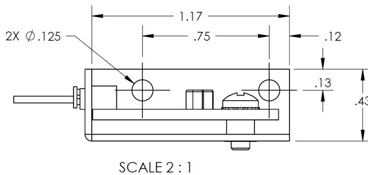
Figure 3-5 Lower paper sensor mounting bracket
