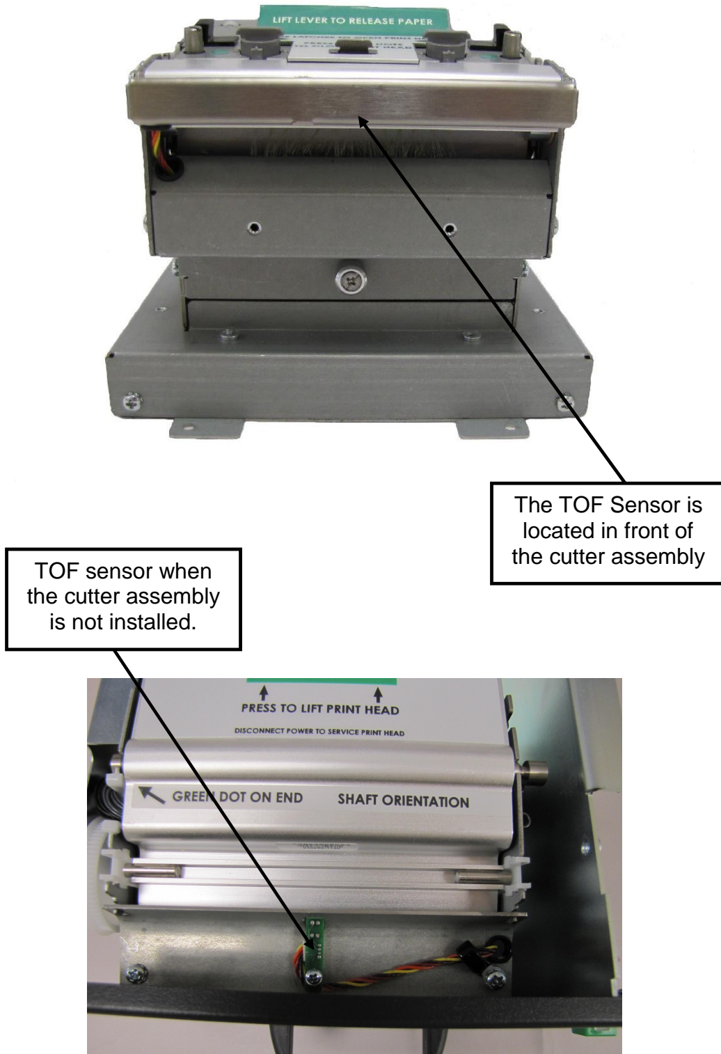
Figure 3-10 TOF (Top-Of-Form) Sensor
