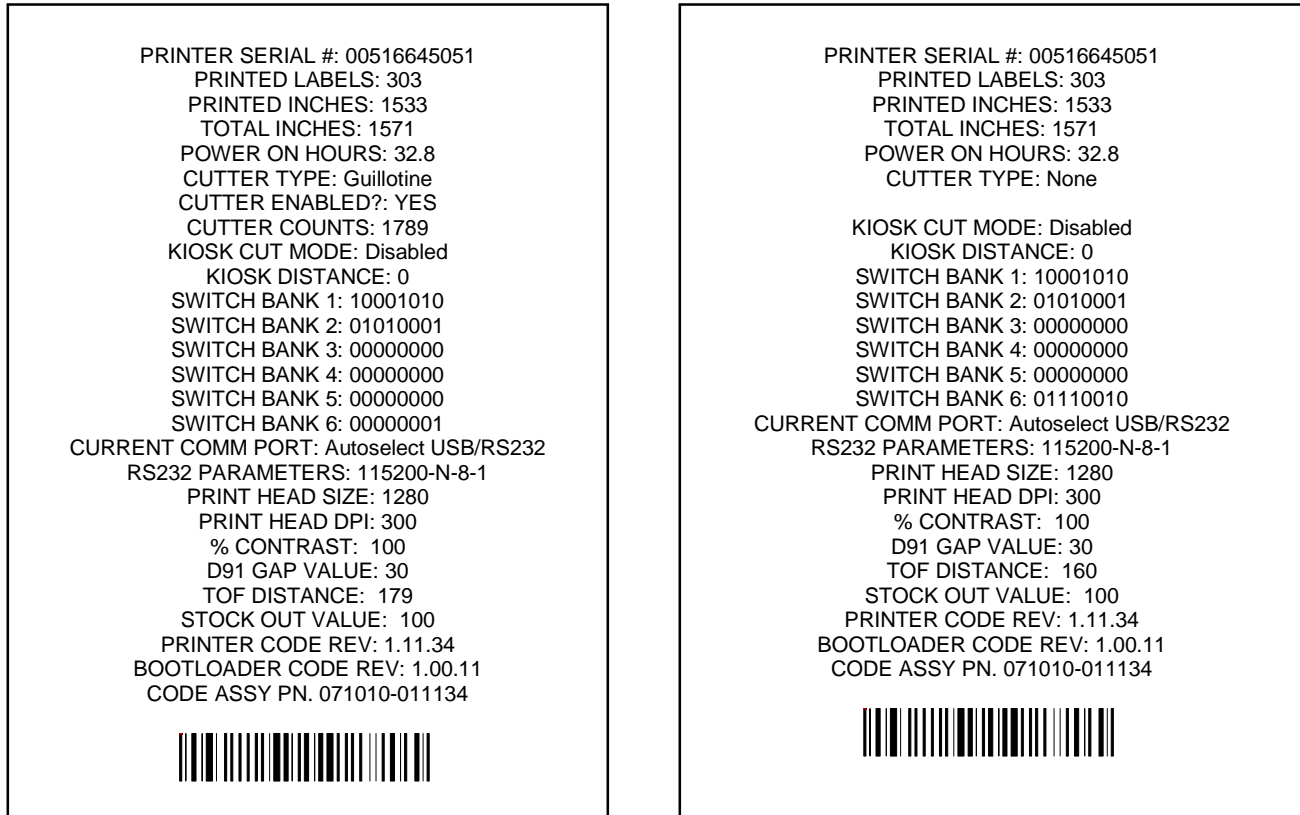
Figure 3-8 Status Label (Examples)
