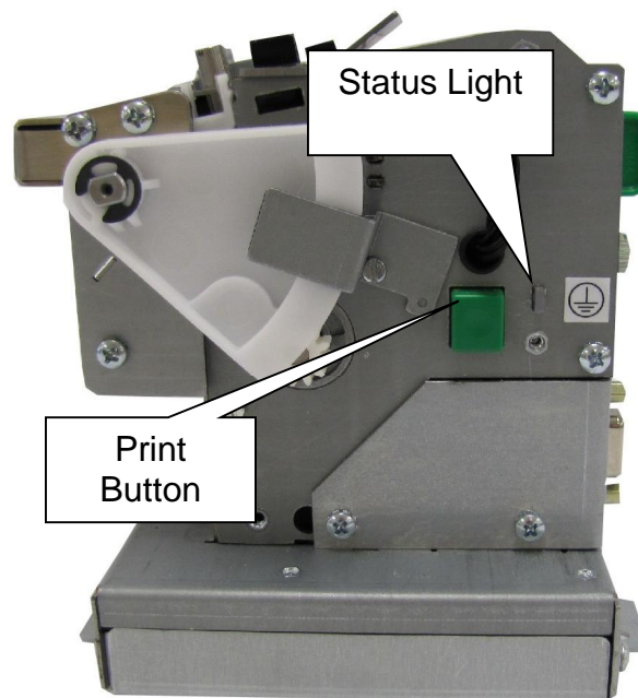
Figure 3-7 Print Button and Status Indicator Light
