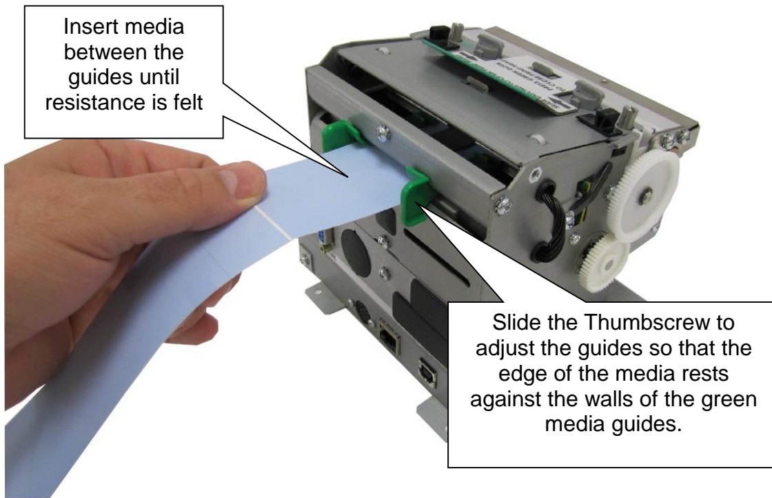
Figure 3-6 Loading Media
