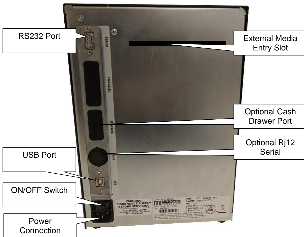
Figure 3-2 Printer Rear Panel
