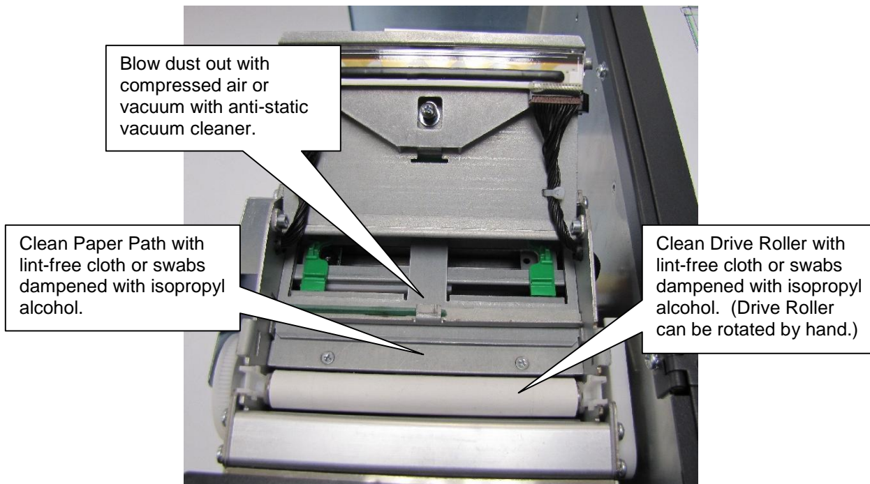
Figure 4-4 Internal Cleaning
