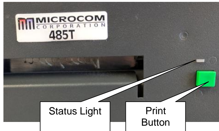
Figure 3-7 Print Button and Status Indicator Light
