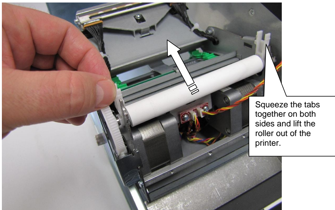
Figure 4-8 Removing the Platen
