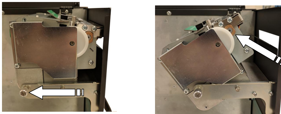
Figure 4-6 Releasing the Print Mechanism
