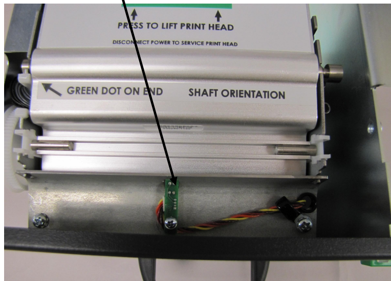
Figure 3-10 TOF (Top-Of-Form) Sensor
