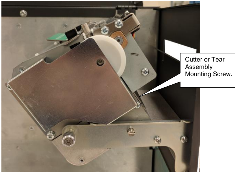
Figure 4-7 Cutter or Tear Assembly Mounting Screw
